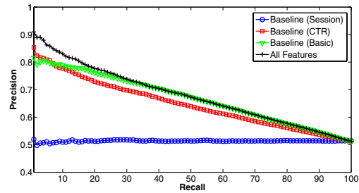
Figure 12: Precision-Recall curve for all algorithms.
