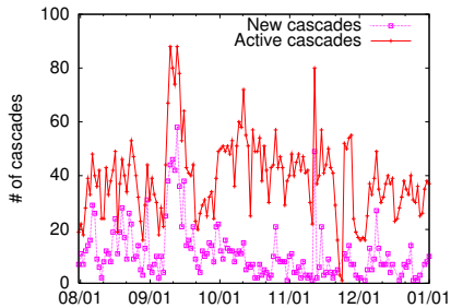
Figure 2: Number of active/new cascades over time.
